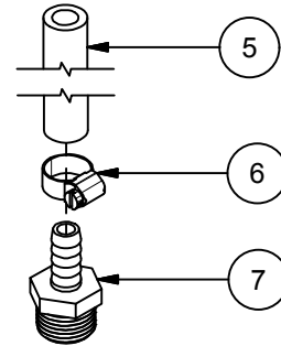
12584 Hose Assembly For Use on 2AC W/ plastic Valve Bracket 3/8" x 15" w/ 1/2"NPT
