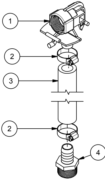
12583 Upper Trough 30" Supply Line Assembly (For All Cattle Units)
